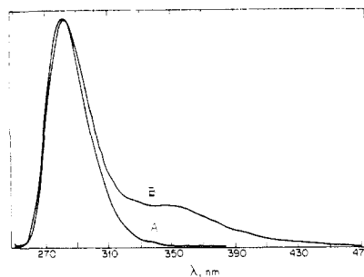
Figure 2. Emission spectra of 322 showing both monomer emission (A; 1.0 \times 10^{-5} M) and excimer emission (B; 1.0 \times 10^{-2} M).
