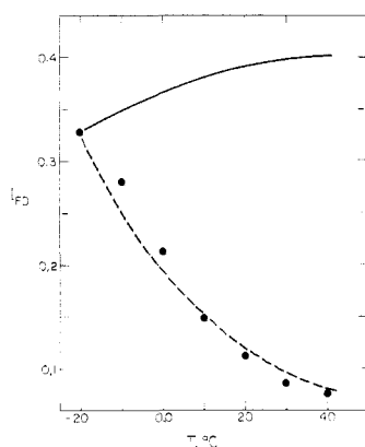
Figure 5. Temperature dependence of excimer fluorescence intensities with the temperature dependence explicitly placed in k_{FD} (—) or k_{ID} (---) observed data (●).
